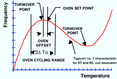
Oven Parameters vs. Stability for SC-cut Oscillator Assuming T_1 - T_{LTP} = 10^\circ\text{C}
